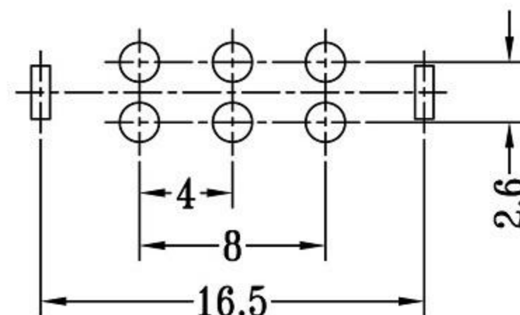
P.C.B LAYOUT BOTTOM VIEW
